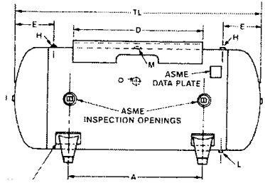
HORIZONTAL WITH PLATFORM
