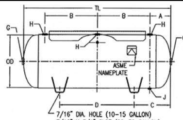
ASME MOBILE TRUCK RECEIVER WITH PLATFORM
